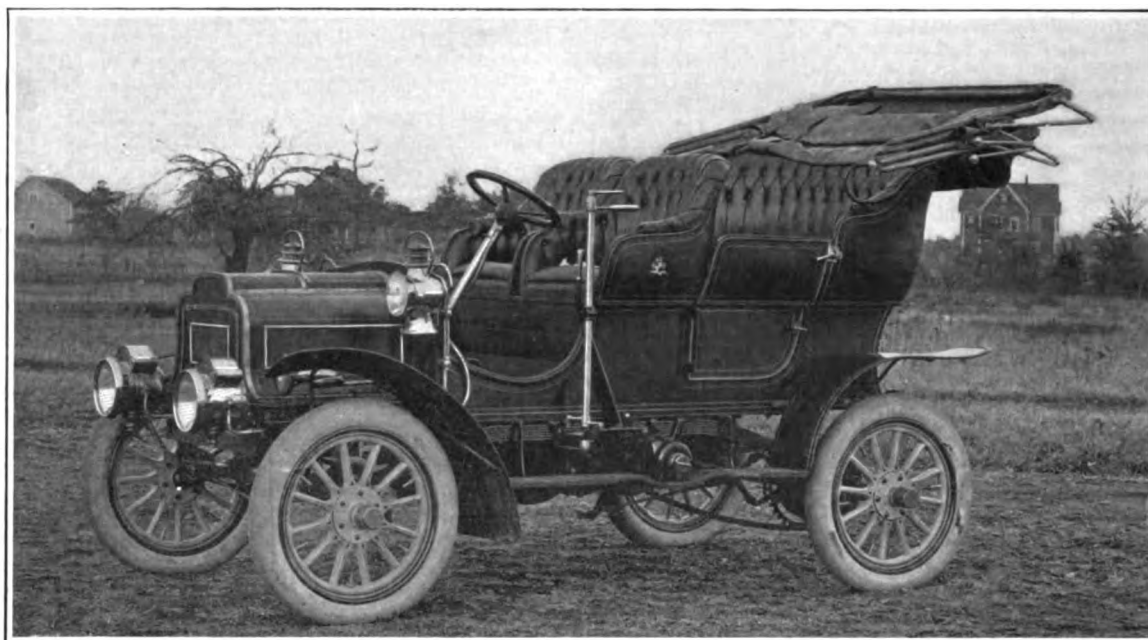
NEW KNOX SIDE ENTRANCE TOURING CAR, WITH TWO-CYLINDER, AIR-COOLED MOTOR AND BONNET FRONT.
